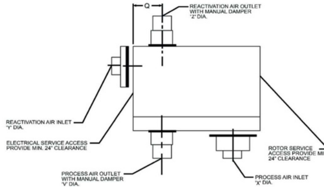
MP UNIT Dimensional Data (Inches)
